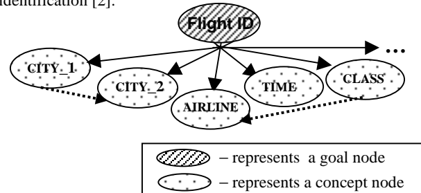
Figure 2. Topology of the BNs for the informational goal Flight_ID .
